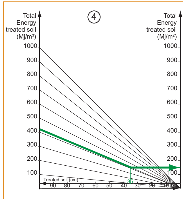
Figure 26: Soil treatment zone – Quadrant of total Energy (/m³ et /m²)
